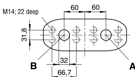
Detail X
